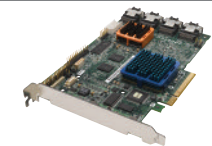
Adaptec RAID 31605 16-port, PCIe, RAID 0, 1, 1E, 5, 5EE, 6, 10, 50, 60
