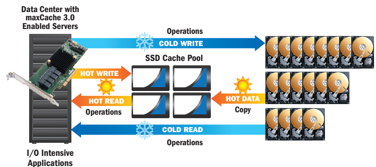
Figure 1. Adaptec maxCache 3.0 Deployment
