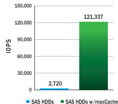
Figure 3. 44x Increase in read caching IOPS with maxCache 3.0
