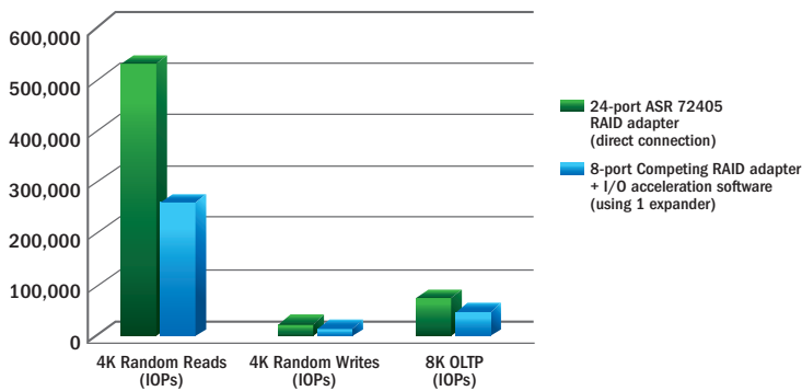
Figure 2. RAID 5 Random Performance (24 SATA SSDs)
