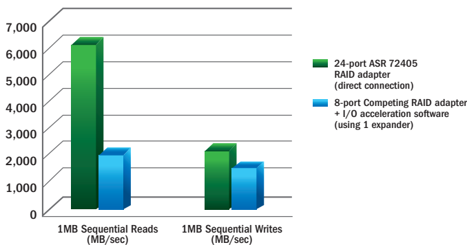
Figure 3. RAID 5 Sequential Performance (24 SATA SSDs)
