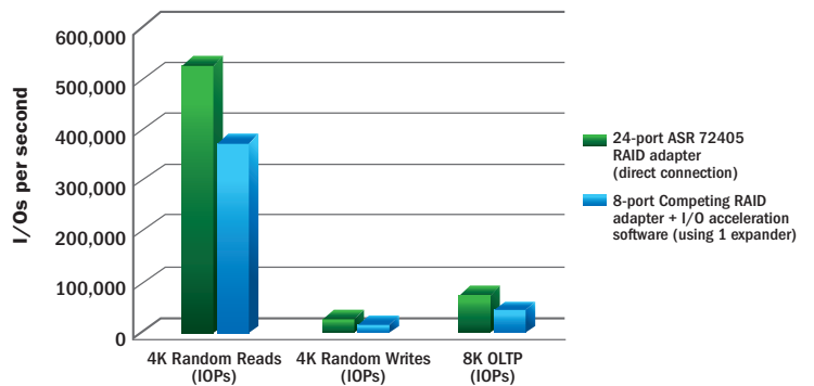
Figure 4. RAID 5 Performance (24 SAS SSDs)
