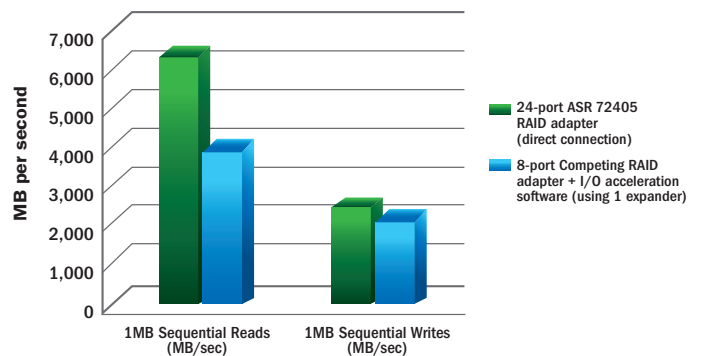
Figure 5. RAID 5 Sequential Performance (24 SAS SSDs)
