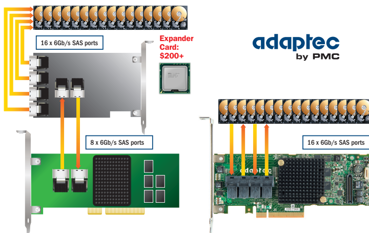
Figure 6. Configuration Complexities and Costs Expanders vs. Direct Connect
