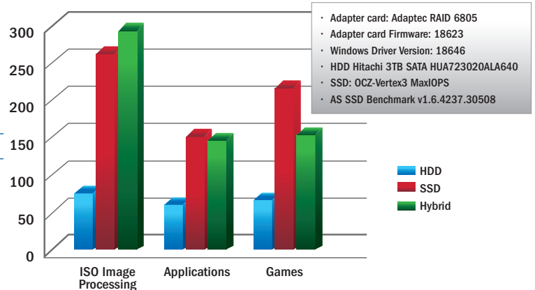
Figure 11. AS SSD Application Performance
