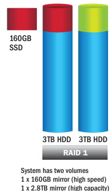
Figure 5. Small Business Server, Hybrid RAID Solution
