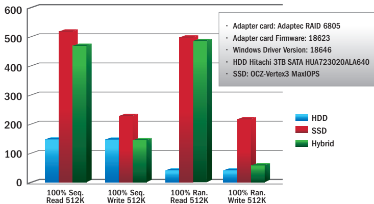
Figure 10. IOMeter Raw Performance
